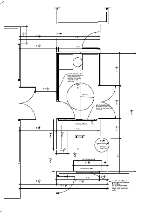
2 AS BUILT RECEPTION AREA W/ NEW GLASS WALL / DOOR AND SLIDING WINDOWS
